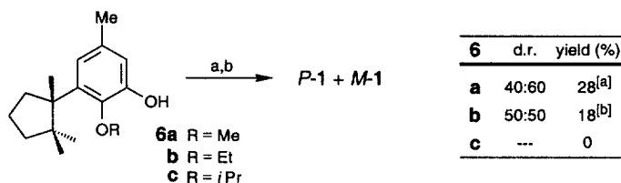
Scheme 2. Oxidative dehydrodimerization of various phenolic precursors 6 to give mastigophorenes A ( P-1 ) and B ( M-1 ). Reaction conditions: a) ( tert -BuO) 2 , C 6 H 5 Cl, reflux; b) BBr 3 , CH 2 Cl 2 , 0 °C. [a] 42% of 3 recovered; [b] 34% of 6b recovered.
