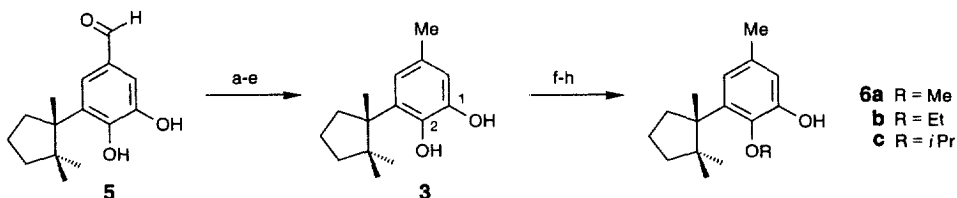
Scheme 1. Synthesis of the monophenolic coupling precursors 6a-c . Reaction conditions: a) \text{Me}_2\text{SO}_4 , \text{K}_2\text{CO}_3 , acetone, rt, 73%; b) \text{LiAlH}_4 , THF, 95%; c) \text{C}_2\text{Br}_2\text{Cl}_4 , \text{Ph}_3\text{P} , \text{CH}_2\text{Cl}_2 ; d) \text{LiAlH}_4 , \text{Et}_2\text{O} , 72%; e) \text{BBr}_3 , \text{CH}_2\text{Cl}_2 , 0 °C, 93%; f) \text{BzlBr} , \text{K}_2\text{CO}_3 , acetone, rt, 90%; g) \text{RI} , \text{Cs}_2\text{CO}_3 , \text{Bzl}(n\text{-Bu})_3\text{NBr} , acetone, a , 97%; b , 85%; c , 65%; h) \text{H}_2 , Pd/C (10%), \text{EtOH}/\text{AcOEt} , 1 atm, rt, 89% (resp. 80%, 75%).
