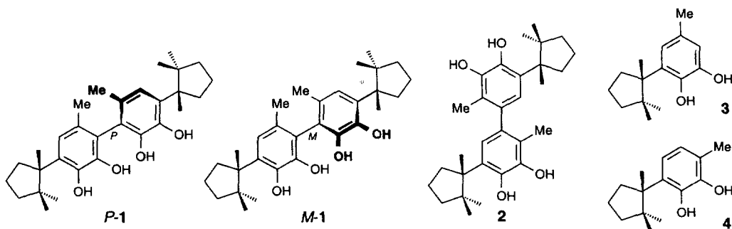
Fig. 1. Natural mono- and dimeric phenolic terpenoids.
